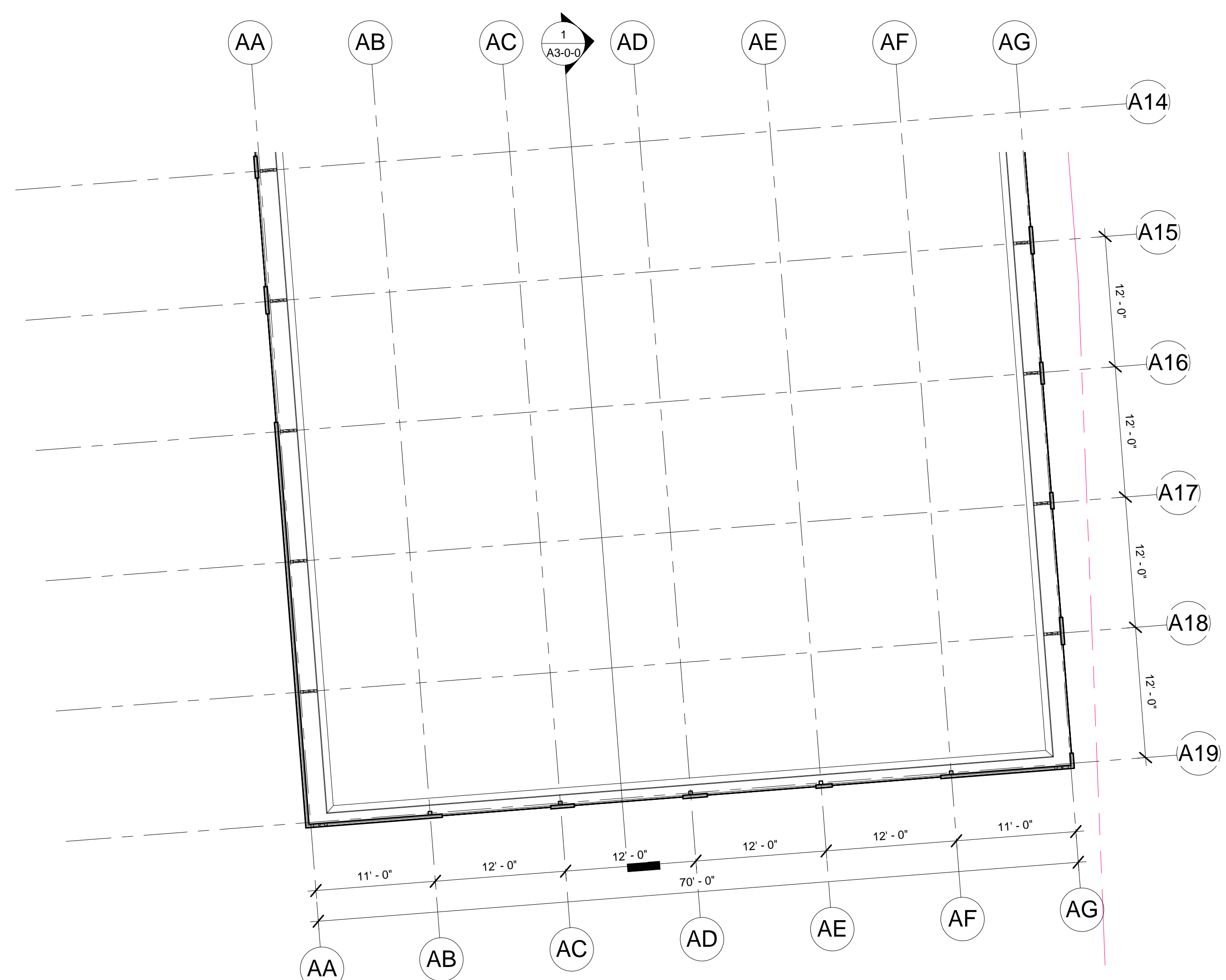
INDOOR RIDING ARENA LEVEL (SOUTH END) 1/8" = 1'-0"
